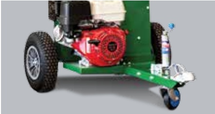
Standard machine with towbar for towing on your property or leg mounting.
